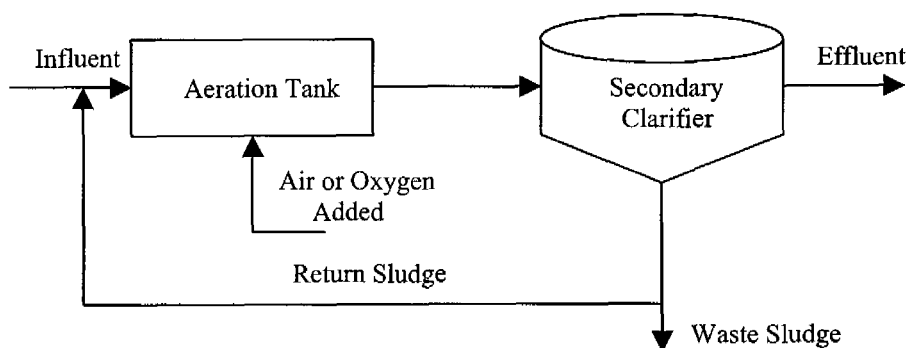
Figure 2: Typical activated sludge process
