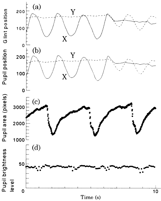
Figure 7: Pupil brightness stabilization and real-time glint and pupil center detection.
