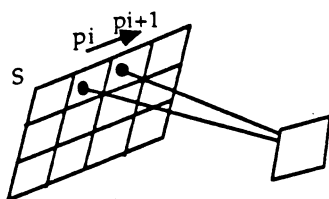
Figure 1. Virtual motions in form-factors computations: linear movement.
