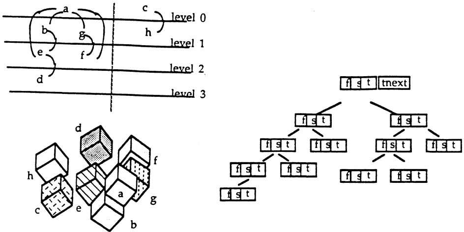
Figure 4. Data Structures of the Algorithm.
