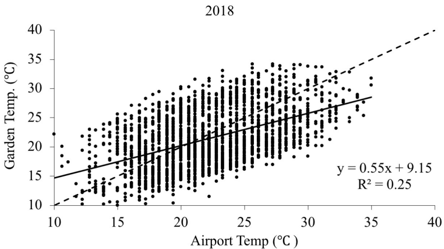
Figure 2: Relationship between measured hourly air temperature at the UST research garden and MSP airport during summer 2018. The solid line is a regression line; the dashed line is a 1:1 line.
