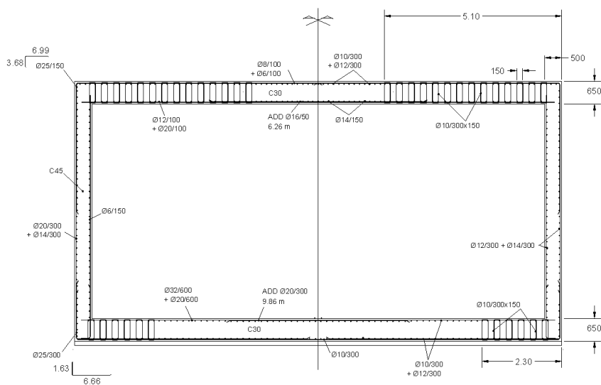
Figure 5: Optimized design of RC box frame for case study 3.
