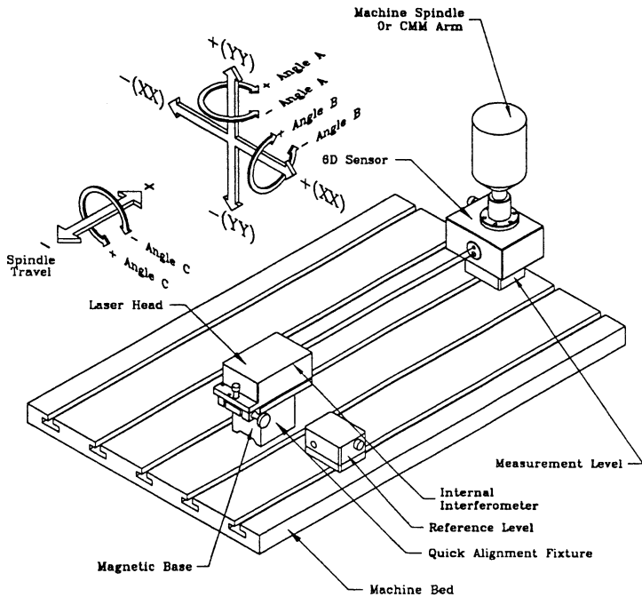
Figure 2. A High Precision Laser Interferometer Setup (Laser head not shown)
