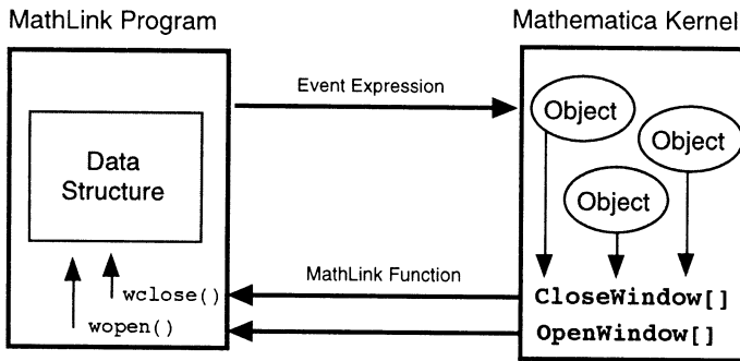
Figure 3: The relation between Object and MathLink Function.
