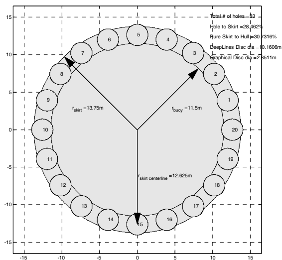
Figure 3: Skirt modelling by using multiple disks.
