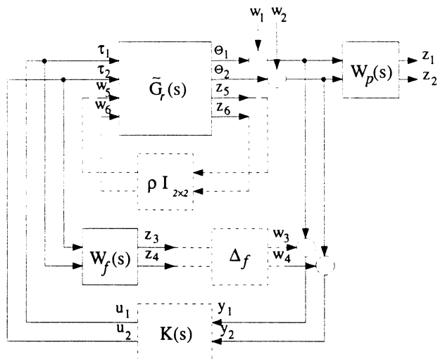
Figure 4: Synthesis Model for Design #2
