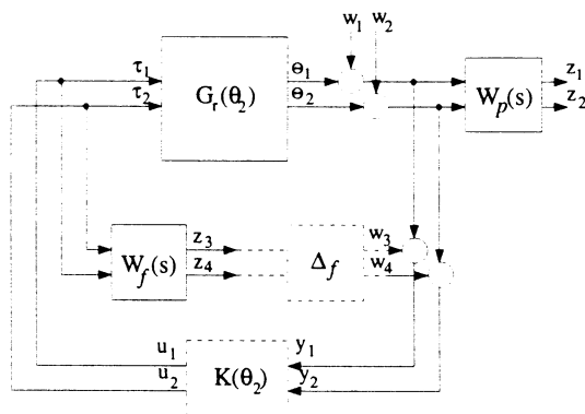
Figure 5: Synthesis Model for Design #3
