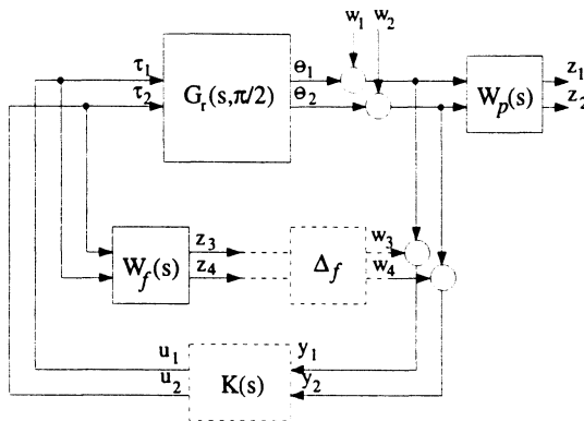
Figure 3: Synthesis Model for Design #1
