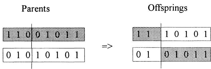
Figure 7: An example of crossover in a classic GA.
