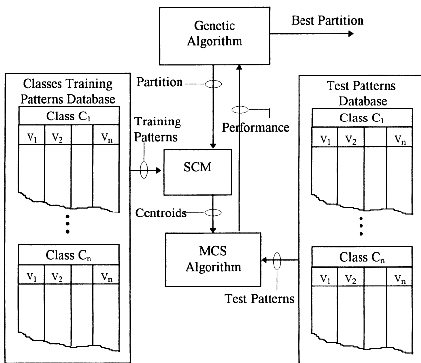
Figure 6: Schematic Diagram of the MCS method
