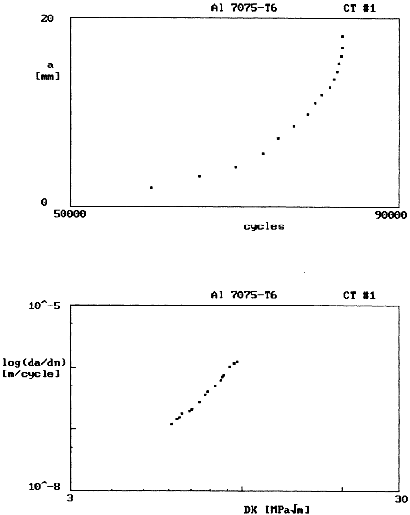
Fig. 13 a-N , da/dN-\Delta K plots for specimen CT #1
