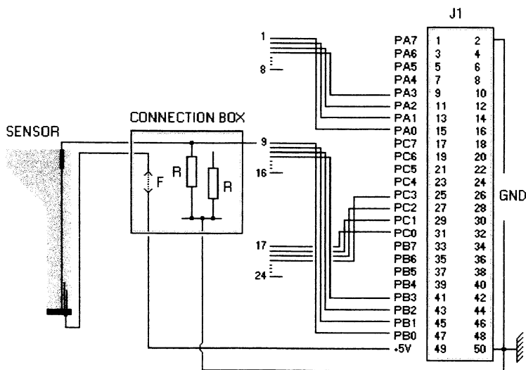
Fig. 5 Hardware layout
