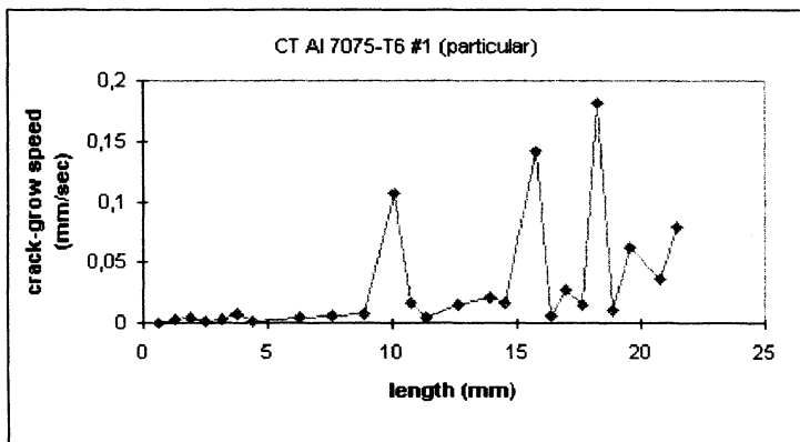
Fig. 9 Crack length and crack-grow speed
