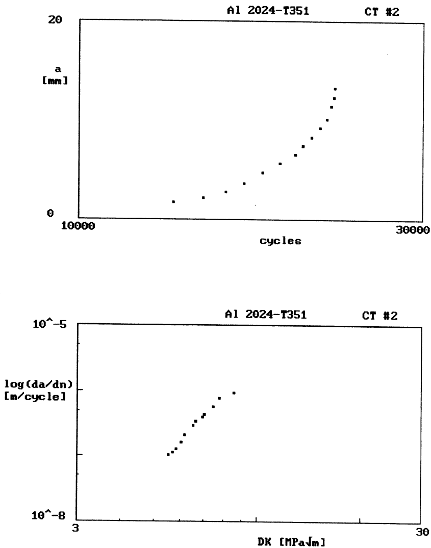
Fig. 14 a-N , da/dN-\Delta K plots for specimen CT #2
