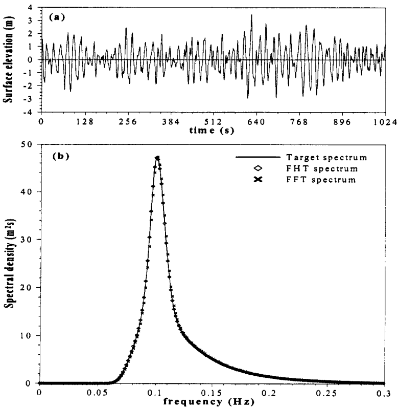
Figure 1: Simulated wave record (a), target spectrum and spectral density function estimated via FHT and FFT (b).
