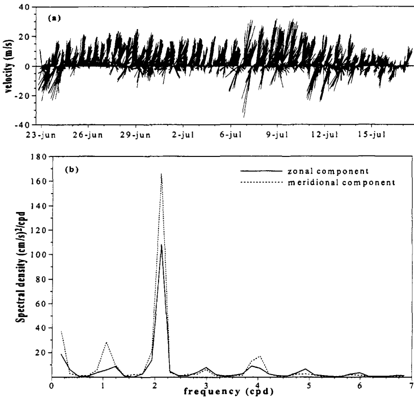
Figure 2: Measured coastal currents record (a) and spectral density functions estimated via FHT for the zonal and meridional velocity components (b).
