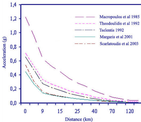
Figure 4: Peak ground acceleration attenuation laws for Greece of a 6Ms earthquake magnitude.
