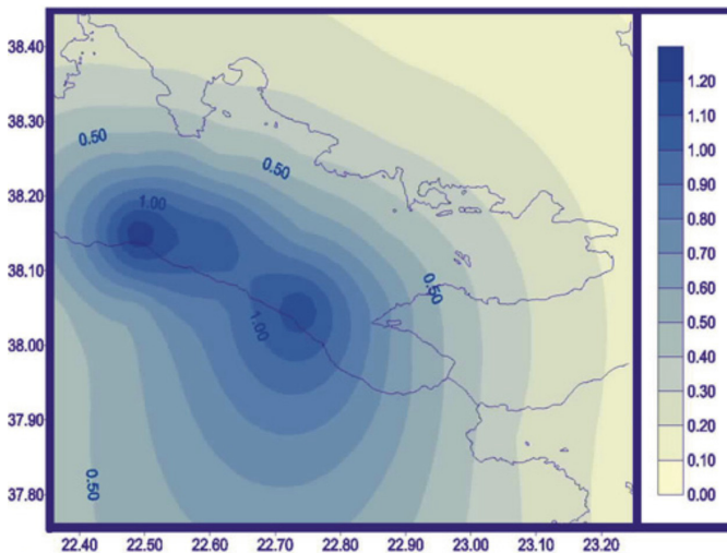
Figure 5: PGA hazard map in units of g (%g) for the region of interest.
