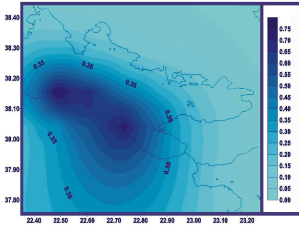
Figure 6: Ia hazard map in units of m/sec (%m/sec) for the region of interest.
