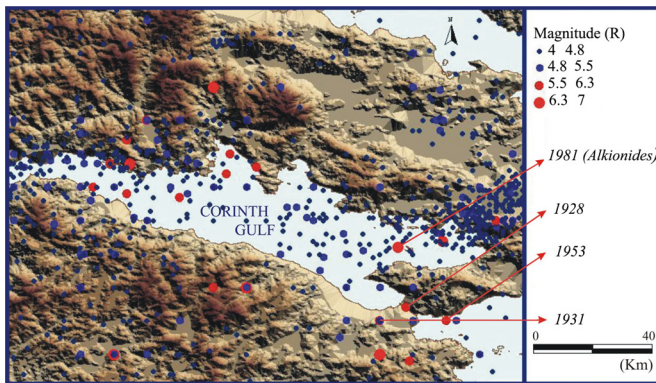
Figure 3: Seismicity map of the Gulf of Corinth, during 1900-2004. Some representative strong earthquake epicenters in the close area of the Corinth Canal have been indicated with arrows.
