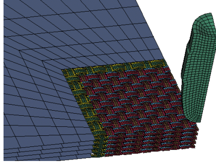
Figure 5: The geometry of the contact interaction between fabric package and the deformable bullet.
