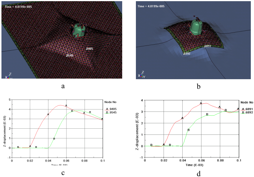
Figure 4: Transverse displacement wave propagation from the center of impact; a– model 30x30 yarns woven patch; b - model 10x10 yarns woven patch; c,d – z-displacement time laws of nodes indicated in figures (a) and (b).
