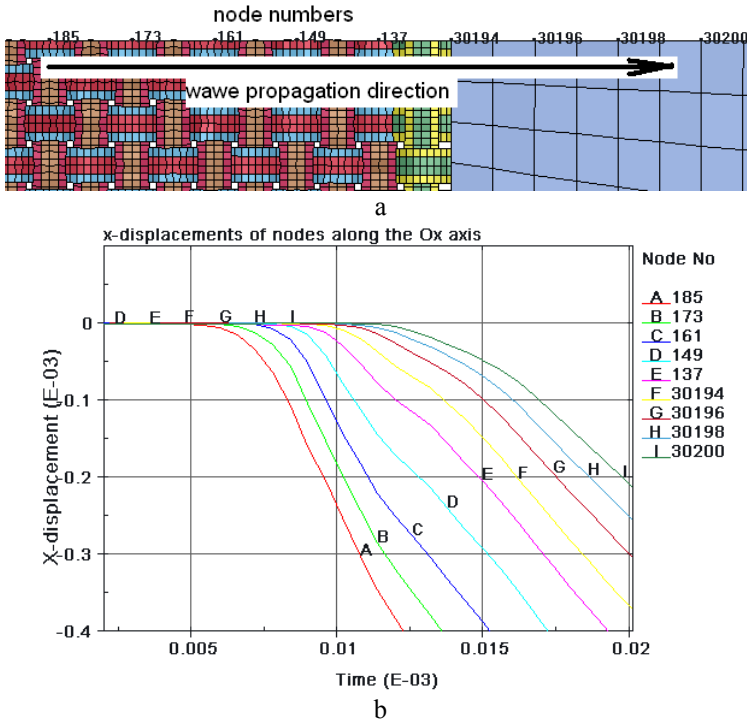
Figure 3: Propagation of the longitudinal component of the impact wave across the tie boundary: numbers of nodes along the wave propagation direction (a) and time laws of longitudinal displacements of nodes (b)
