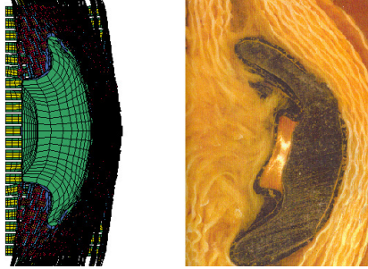
Figure 7: Impact of a full metal jacket bullet against a multilayer fabric (bullet stopped): (a)–simulation; (b)–experiment (photo taken from the circular of Twaron textiles).
