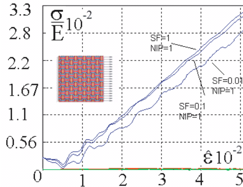
Figure 2: The relationships of the longitudinal strain \sigma/E in a yarn against the relative elongation \hat{\epsilon} of the at different values of the slave contact stiffness scale multiplier SFS
