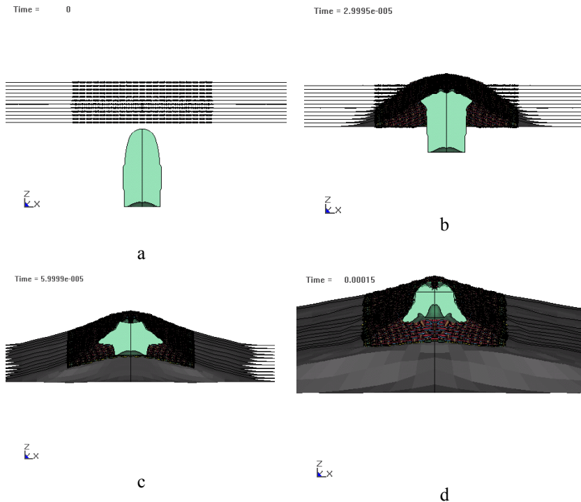
Figure 6: The hold-up of a lead bullet BALLE22 in a 12 layer fabric package.
