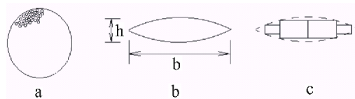
Figure 1: Circular cross-section of a free yarn (a); cross-section of an interwoven yarn (b); cross-section of an interwoven yarn approximated by rectangular cross-sections of four shell elements (c).
