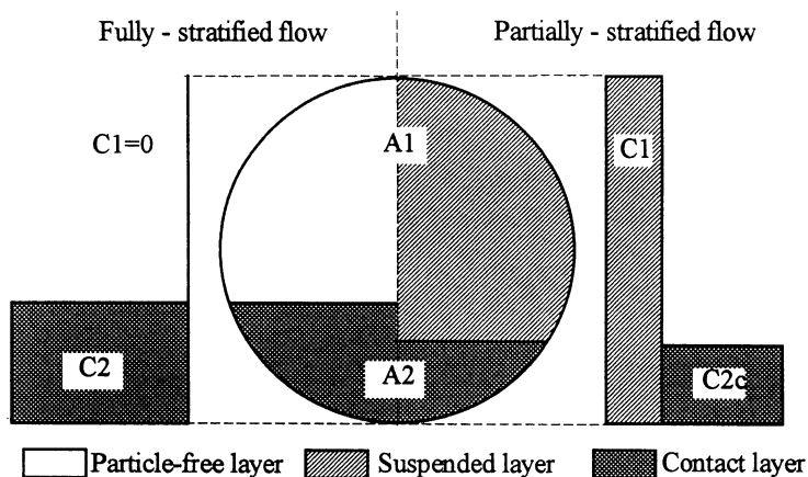
Figure 1: Schematic cross-section for two-layer model.
