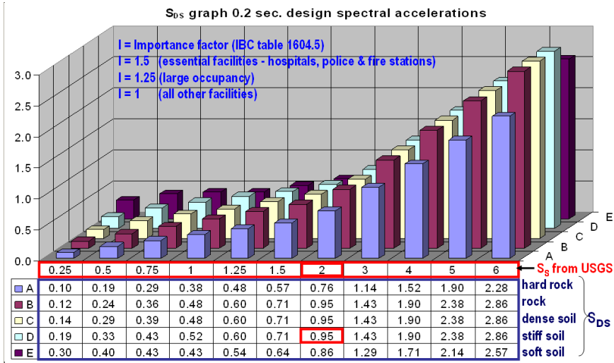
Figure 6: S DS graphs. (Site classes A-E, default site class D used.)
