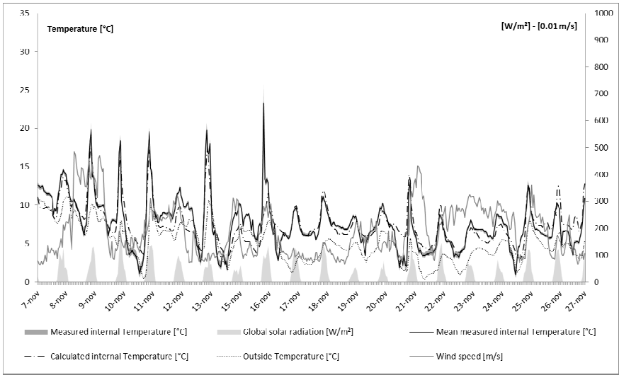
Figure 7: 7–27 November calibration.
