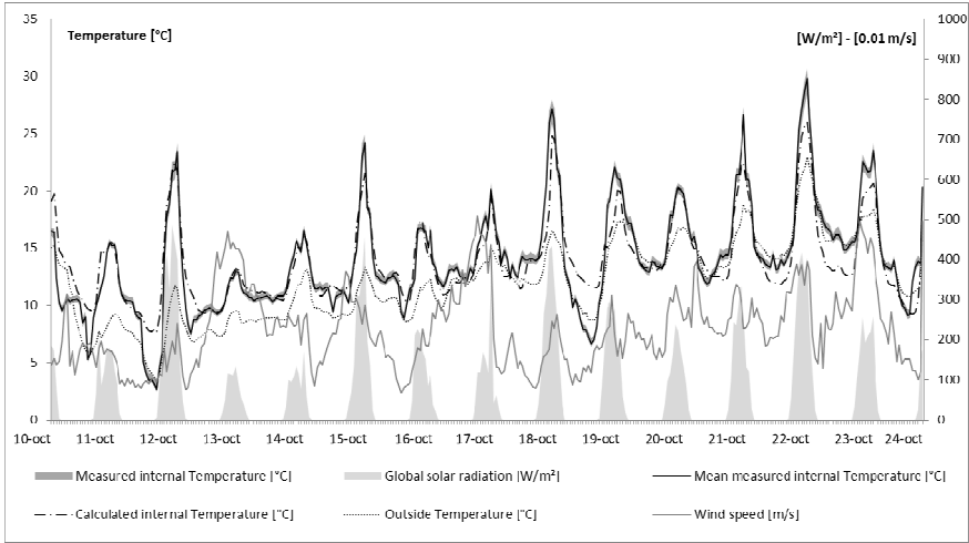
Figure 6: 10–24 October calibration.
