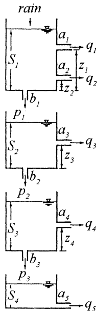
Figure 1: Tank model
