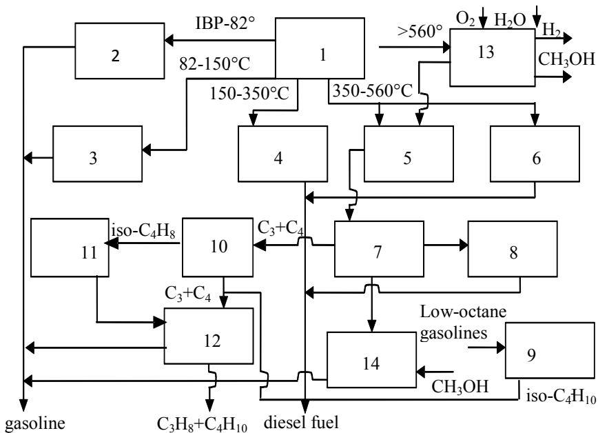
Figure 3: The scheme of the residueless oil refining: 1. preliminary distillation, 2. isomerization, 3. reforming, 4. hydrorefining, 5. hydrocracking, 6. hydrocracking, 7. catalytic cracking, 8. hydrogenation, 9. hydroisomerization, 10. isobutylene separation, 11. hydrogenation of isobutylene, 12. alkylation, 13. coking + gasification + methanol production, 14. esterification.
