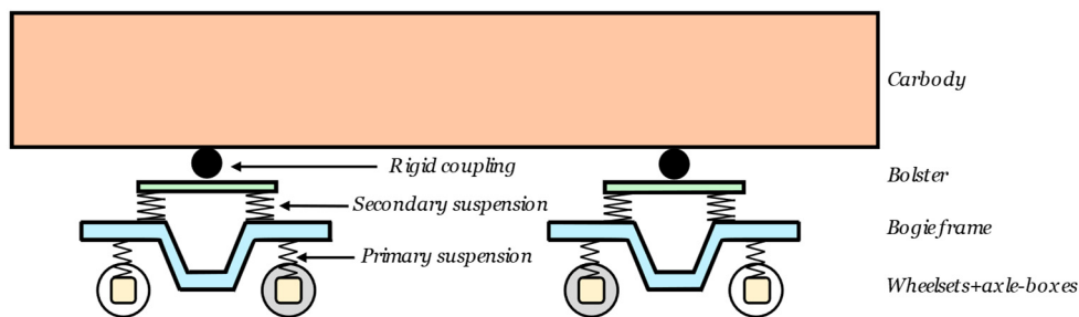
Figure 1: Sketch of the MB model architecture (powered wheelsets are coloured in grey).
