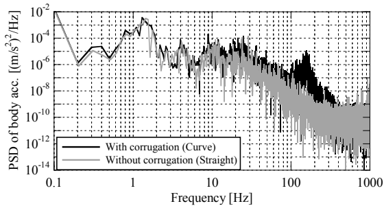
(b) PSD of acceleration of vehicle body
